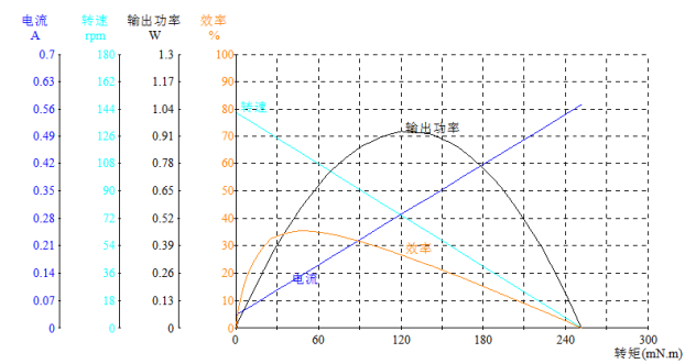
Model: WL-27RS3700124500-27K
