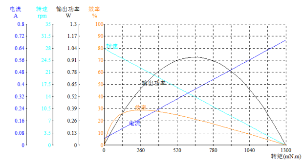
Model: WL-27RS3700126000-210K
