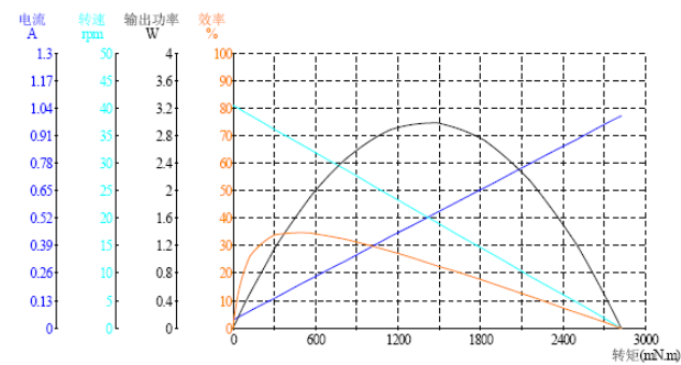
Model: WL-33RS35250247000-174K
