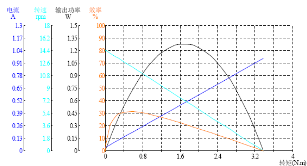
Model: WL-33RS35250124500-312.5K
