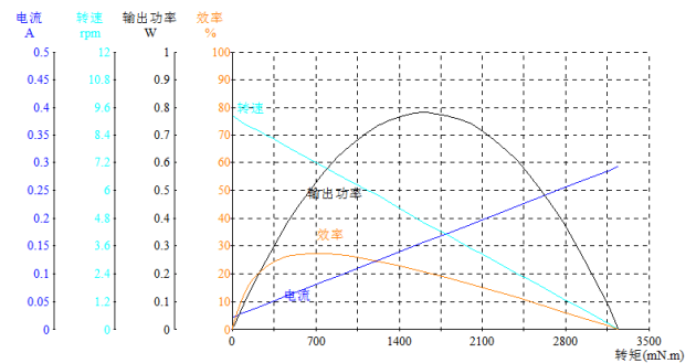
Model: WL-65SS5200244500-450K
