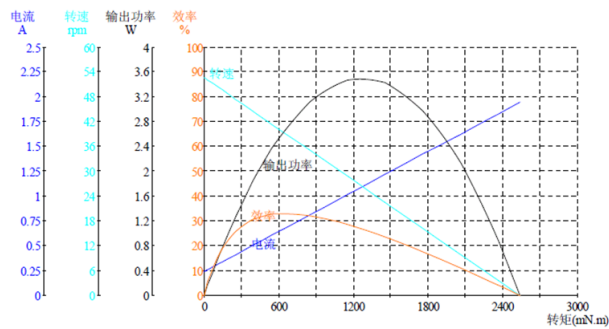
Model: WL-65SS5200128000-135K
